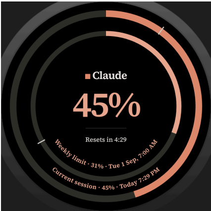
4a Claude
