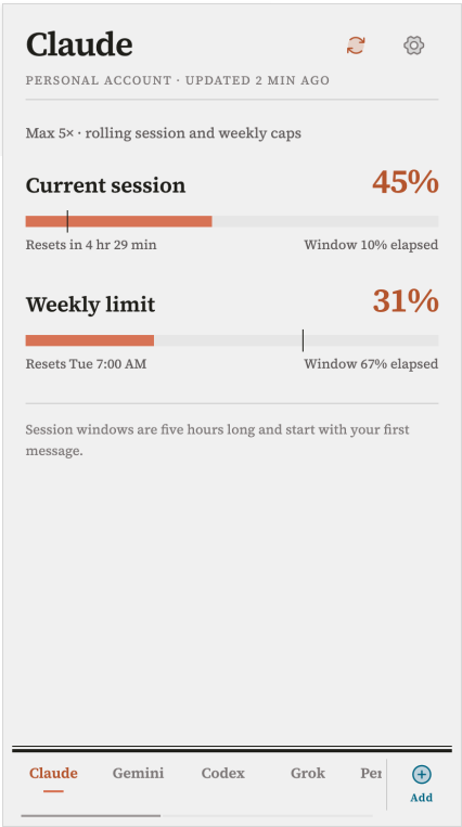
4a Claude
